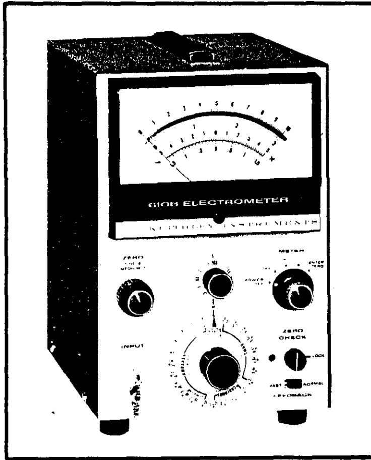
FIGURE 1. Keithley Instruments Model 610B Electrometer.
